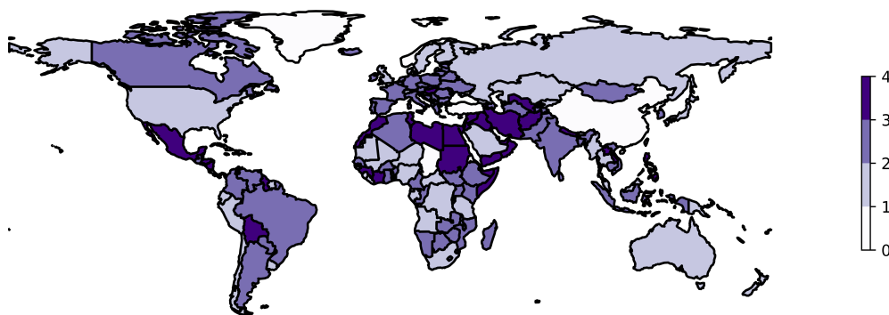
Figure 11: Worldwide availability of vaccines developed using non-replicating viral vectors. This figure reflects the number of vaccines using non-replicating viral vectors that were available in each country as of October 18, 2022. These data are retrieved from Our World in Data ( 1115 ) and plotted using geopandas ( 1159 ). See https://greenelab.github.io/covid19-review/ for the most recent version of this figure, which is updated daily. Note that this figure draws from a different data source than Table 4 and does not necessarily include data for every vaccine developed within this category.
