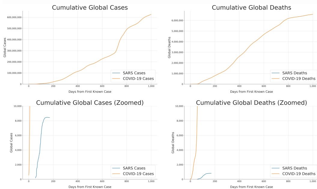
Figure 3: Cumulative global incidence of COVID-19 and SARS. As of October 18, 2022, 625,797,917 COVID-19 cases and 6,570,892 COVID-19 deaths had been reported worldwide since January 22, 2020. A total of 8,432 cases and 813 deaths were reported for SARS from March 17 to July 11, 2003. SARS-CoV-1 was officially contained on July 5, 2003, within 9 months of its appearance (730). In contrast, SARS-CoV-2 remains a significant global threat nearly two years after its emergence. COVID-19 data are from the COVID-19 Data Repository by the Center for Systems Science and Engineering at Johns Hopkins University (731, 732). SARS data are from the WHO (733) and were obtained from a dataset on GitHub (734). See https://greenelab.github.io/covid19-review/ for the most recent version of this figure, which is updated daily.
